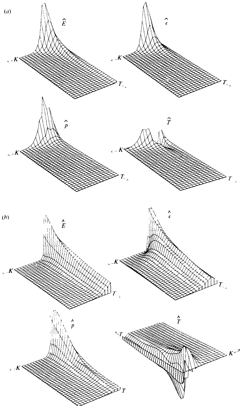
FIGURE 5. Spectral distribution of the kinetic energy \hat{E} , pressure \hat{p} , dissipation \hat{\epsilon} and transfer rate \hat{T} vs. wavenumber ( k = K , 3 \leq k \leq 31 ) and time ( t = T , 0 \leq t \leq 1.6 ) for (a) run I4 and (b) run I1.
