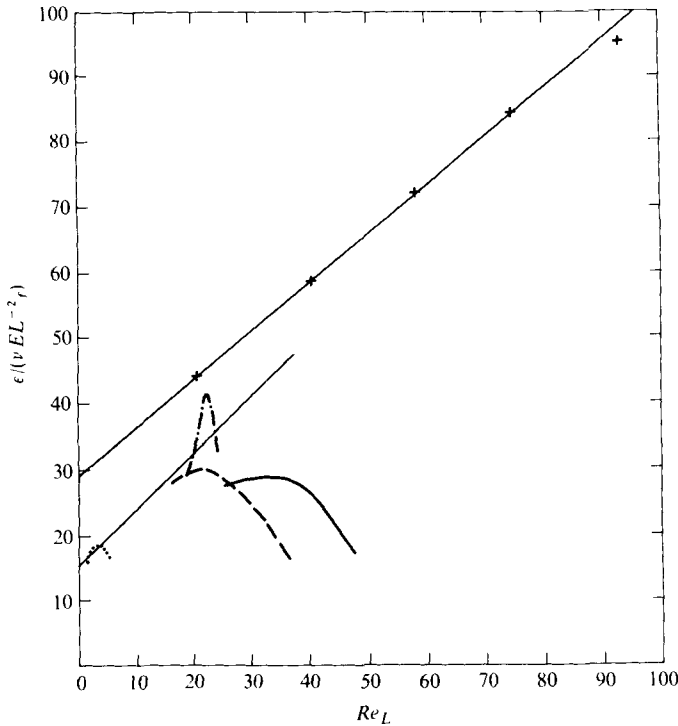
FIGURE 18. Normalized dissipation vs. Reynolds number. —, I1 ; ---, I2 ; — · —, I3 ; ·····, I4 ; +, Herring (1973); —, equation (18), B_1 + B_2(\frac{3}{2})^{\frac{1}{2}} Re_L .
