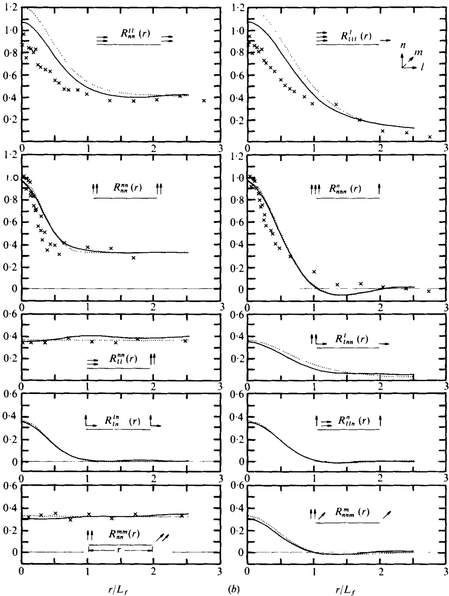
FIGURE 14. Fourth-order two-point velocity correlations normalized by \frac{1}{3}(u_1^4 + u_2^4 + u_3^4) at time t = 0.2 vs. normalized distance for (a) run I3 and (b) run I1. The crosses represent the experimental results of Uberoi (1953). The dotted curves are the predictions from second-order correlations assuming normality.
