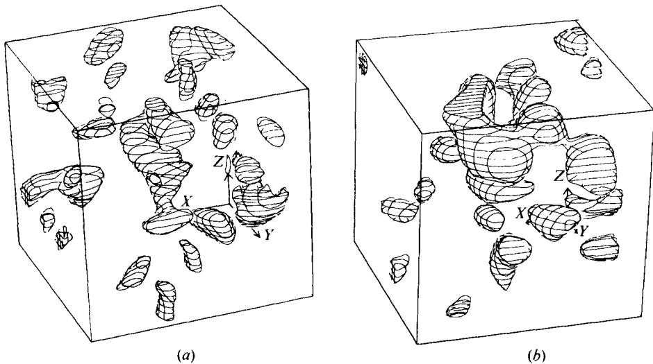
FIGURE 4. Isosurfaces of (a) kinetic energy E and (b) pressure p in real space (x_1, x_2, x_3) = (X, Y, Z) for run I1 at time t = 0.2 . Inside the 'clouds' E \geq 3.365 = \frac{1}{2}E_{\max} and p \leq -1.431 = \frac{1}{3}p_{\min} .
