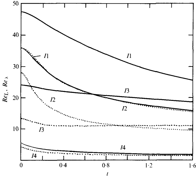
FIGURE 1. Reynolds numbers vs. time. —, Re_L ; ·····, Re_\lambda .
